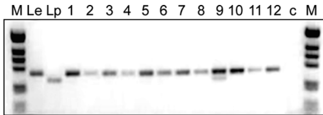
Fig. 3 Identification of chromosome IX as the carrier of the Lycopersicon esculentum ( Le ) and its wild relative L. pennellii ( Lp ) allele of E325111. The polymorphism between Le and Lp is revealed by restriction digestion with AluI . Lanes 1–12 Pools of introgression lines, each representing introgressions in single chromosomes. The complete set of 12 tomato chromosomes covering the Le chromosomes (from 1 to 12) was used. c Control PCR without DNA, M 1-kb size marker (GibcoBRL, Gaithersburg, Md.)
